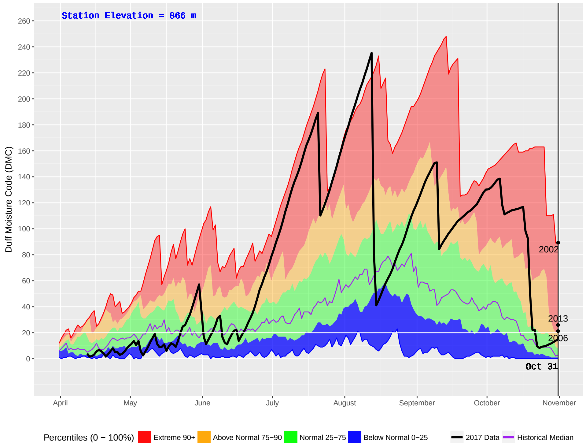
NICOLL (393) : Historical (1981–2016) and Current (2017) Noon Duff Moisture Code (DMC)
